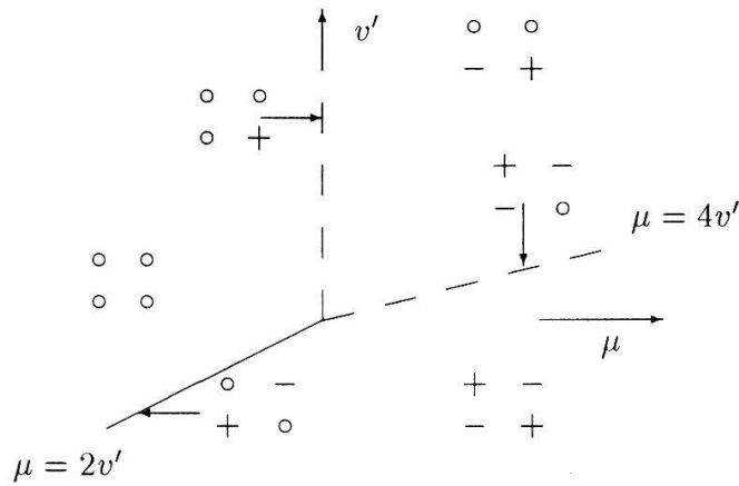
Figure 4: Zero-temperature phase diagram of H_{t-J}(0,0) for v = J
